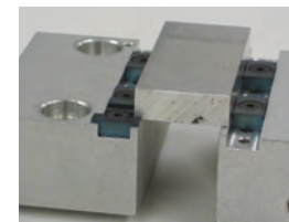
Soft Jaws
