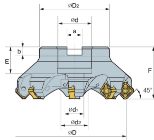
2" - 5" (coolant hole)
