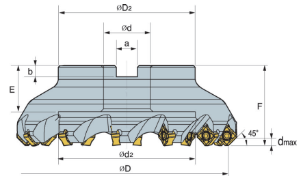
6" - 8" (no coolant hole)
