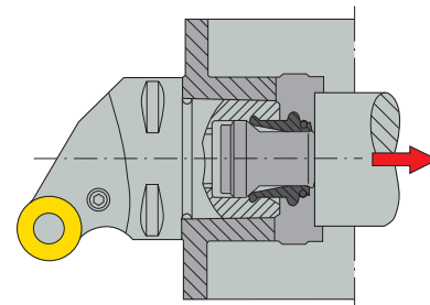
Clamping segments
