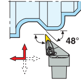
C.-DVJNR/L KAPR = 93,0 °
