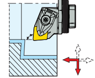
GL...DCLNR/L KAPR = 95,0 °
