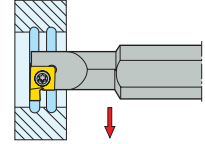
SNR/L KAPR = 90,0 °
