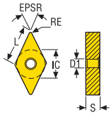
DNMA
