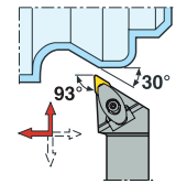
DDJCR/L...JETI KAPR = 93,0°
